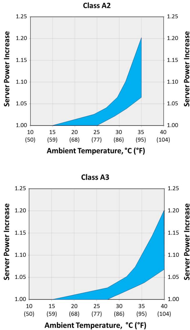
Figure 2.6 Server power increase (Class A3 is an estimate) versus ambient temperature for Classes A2 and A3.
