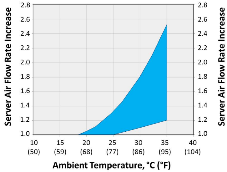
Figure 2.7 Server flow rate increase versus ambient temperature increase.
