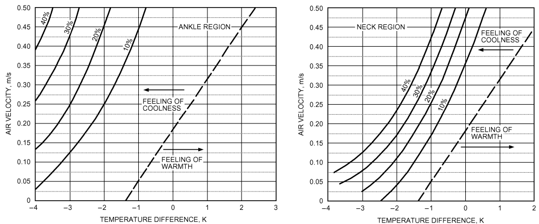
Figure 1.10 Percentage of Occupants Objecting to Drafts in Air-Conditioned Rooms 2013E Ch 20 Fig 111
