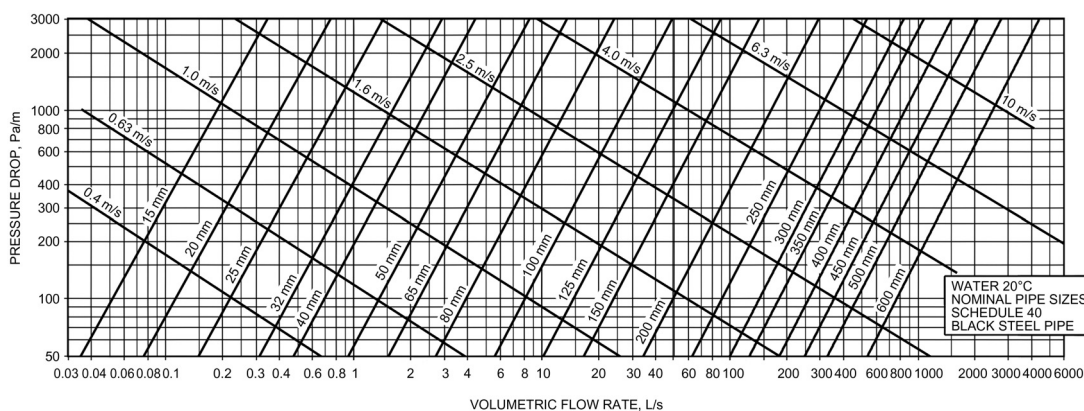
Figure 3.10 Friction Loss for Water in Commercial Steel Pipe (Schedule 40) 2013F, Ch 11, Fig. 41
